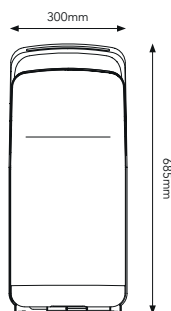
FRONT ELEVATION
